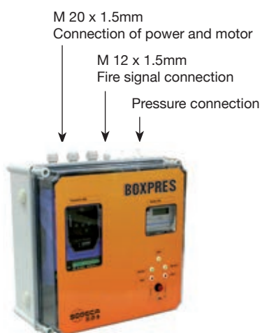
Stuffing-box for cable input to equipment Size 1
