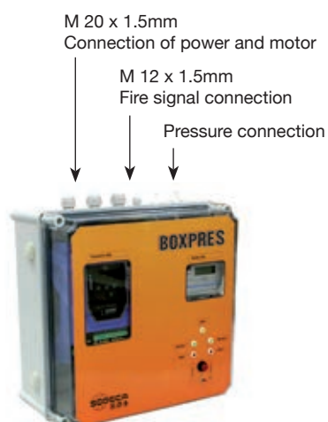
Stuffing-box for cable input to equipment Size 2
